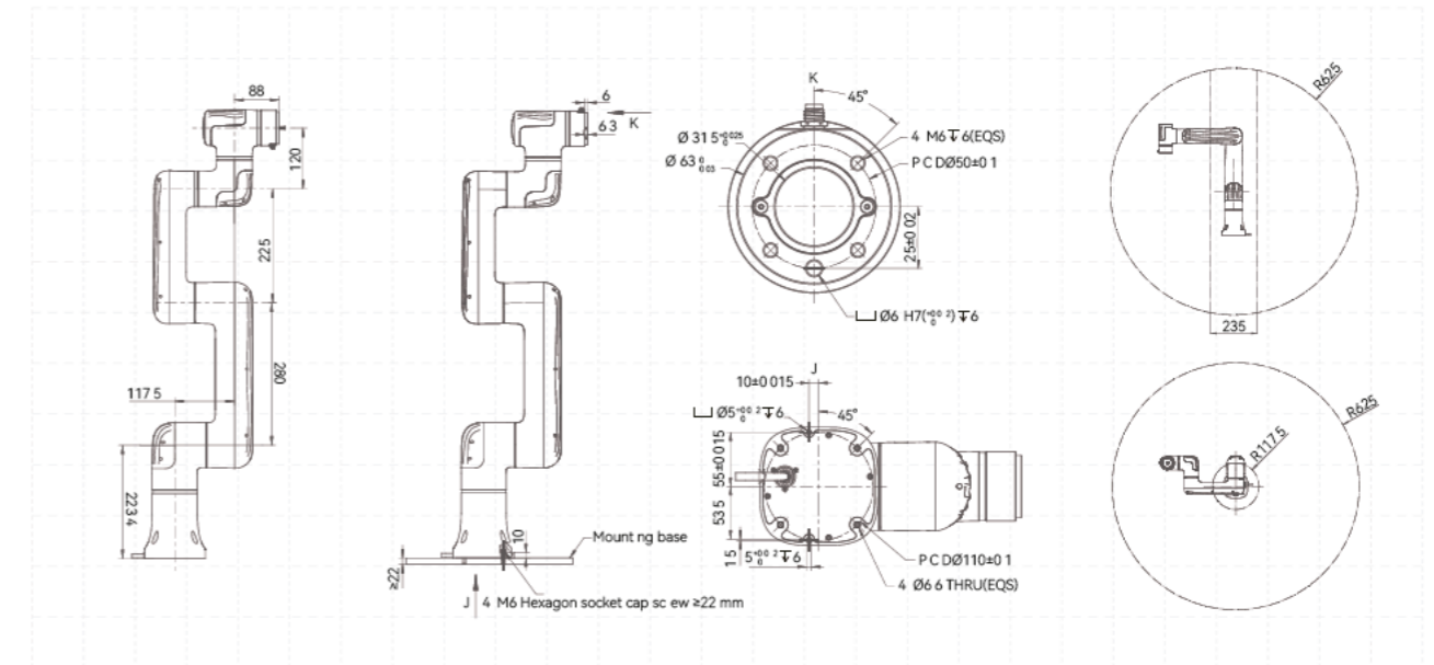
Overall dimension diagram Mounting hole diagram Motion range diagram
